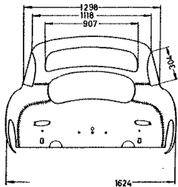
Width of rear door jamb
